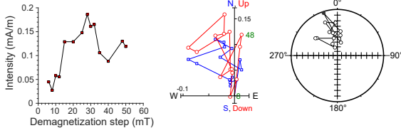
397-U1587B-47X-3, 138 cm | 426.08 m CSF-A | SRM data
