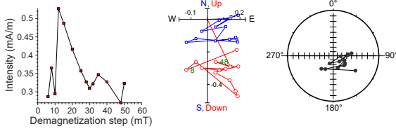
397-U1587B-49X-3, 104 cm | 445.17 m CSF-A | SRM data
