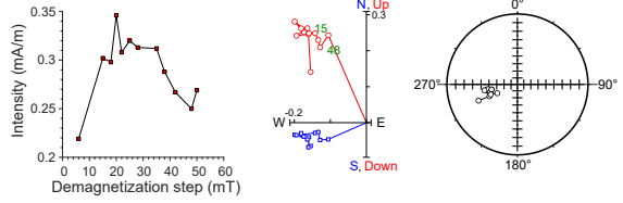
397-U1587B-50X-5, 105 cm | 457.89 m CSF-A | SRM data
