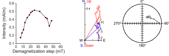
397-U1587B-47X-3, 34 cm | 425.04 m CSF-A | SRM data
