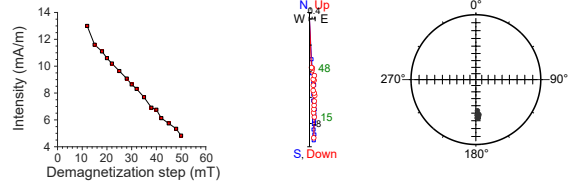
397-U1587B-51X-1, 89 cm | 461.41 m CSF-A | SRM data
