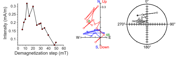
397-U1587B-48X-4, 42 cm | 436.32 m CSF-A | SRM data
