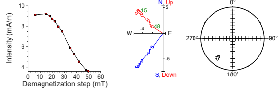
397-U1587B-51X-3, 118 cm | 464.7 m CSF-A | SRM data
