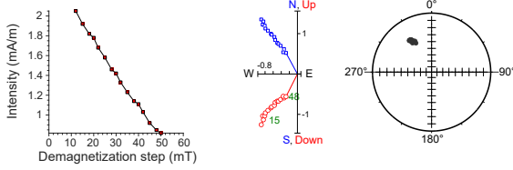
397-U1587B-50X-2, 77 cm | 453.1 m CSF-A | SRM data
