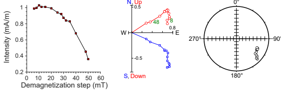
397-U1587B-49X-2, 113 cm | 443.75 m CSF-A | SRM data
