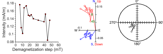
397-U1587B-46X-W, 100 cm | 417.52 m CSF-A | SRM data
