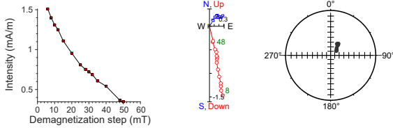
397-U1587B-49X-5, 118 cm | 448.32 m CSF-A | SRM data
