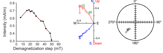
397-U1587B-48X-2, 67 cm | 433.58 m CSF-A | SRM data
