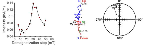
397-U1587B-48X-3, 98 cm | 435.38 m CSF-A | SRM data
