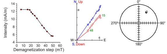
397-U1587B-51X-2, 41 cm | 462.43 m CSF-A | SRM data
