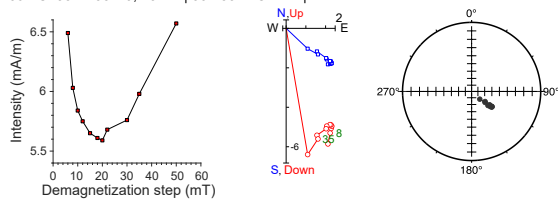
397-U1587B-58X-3, 45 cm | 531.85 m CSF-A | SRM data
