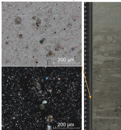
Nannofossil ooze with diatoms and clay U1385G-12H-6, 50 cm
