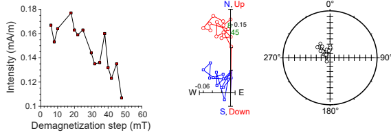
397-U1385G-18X-4, 74 cm | 160.03 m CSF-A | SRM data
