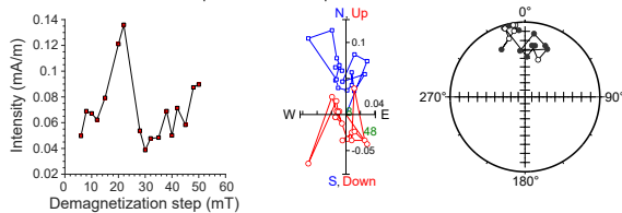
397-U1385G-26X-3, 72 cm | 236.14 m CSF-A | SRM data
