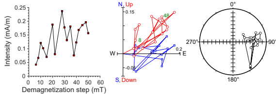
397-U1385G-25X-4, 68 cm | 227.9 m CSF-A | SRM data
