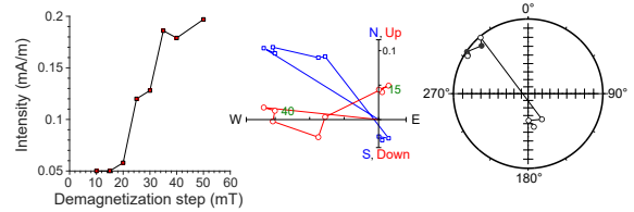
397-U1385G-27X-3, 25 cm | 245.38 m CSF-A | SRM data
