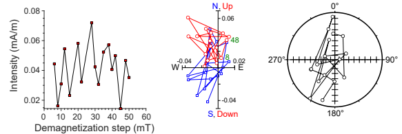
397-U1385G-29X-5, 90 cm | 268.44 m CSF-A | SRM data
