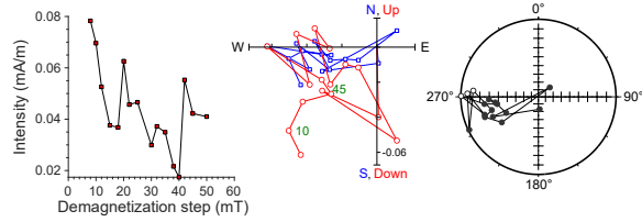
397-U1588A-48X-4, 67 cm | 347.399 m CSF-B | SRM data
