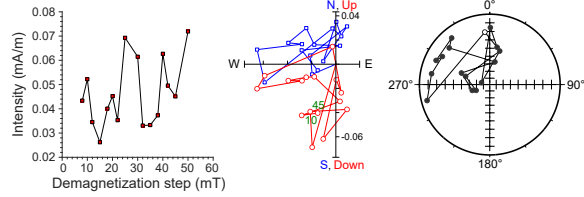
397-U1588A-46X-2, 47 cm | 335.404 m CSF-B | SRM data
