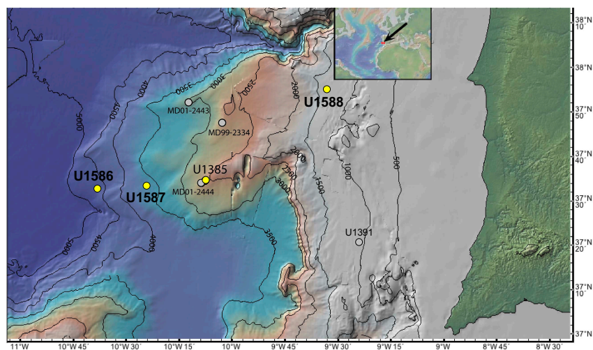
Figure F1. Bathymetry of the Promontório dos Príncipes de Avis (PPA) showing the locations of the four sites (U1586, U1587, U1385, and U1588) drilled during Expedition 397, Marion Dufrenoy (MD) piston cores, and IODP Site U1391. Site U1385 was occupied previously during Expedition 339, as was Site U1391. The map is modified from Hodell et al. (2015) and was made with GeoMapApp ( http://www.geomapapp.org ) using the bathymetry of Zitellini et al. (2009).
