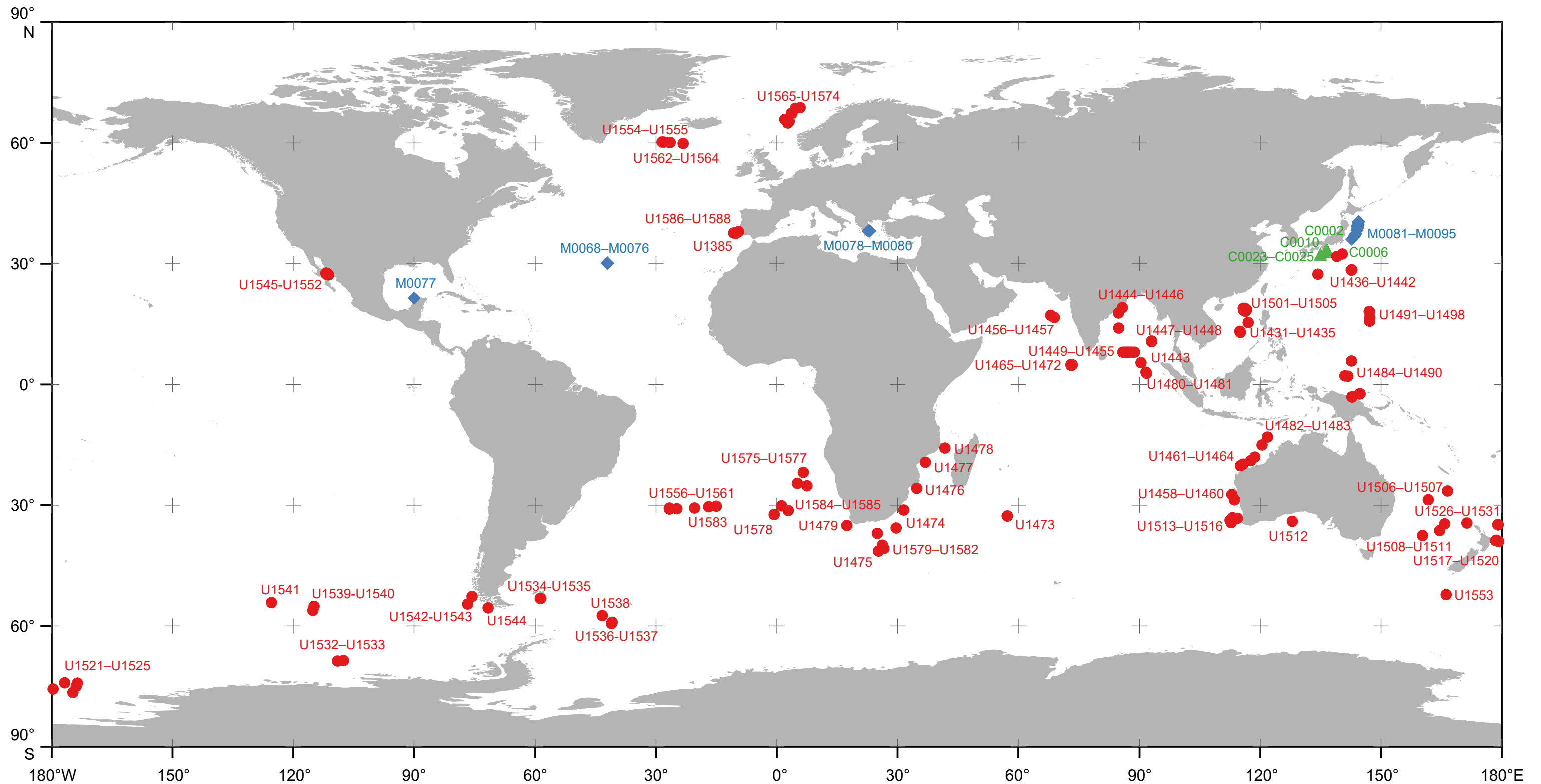
IODP Expeditions 349–372, 374–376, 378–386, 390–393, 396–397, Sites C0002, C0006, C0010, C0023–C0025 (▲), M0068–M0095 (◆), U1385, U1431–U1588 (●)
