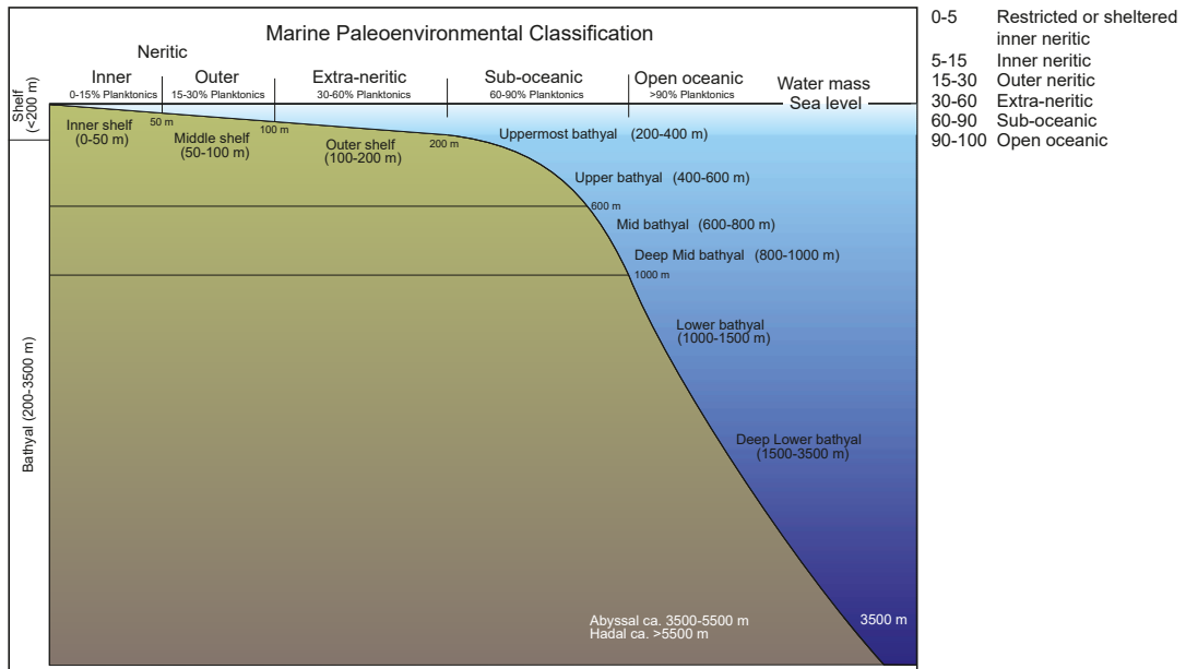
Oceanicity (Watermass): Based on planktonic foraminiferal abundance (%) relative to all foraminifera in the 150-500 µm sediment size fractions of washed residues.
