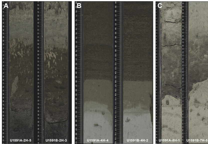
Subunit Ia
