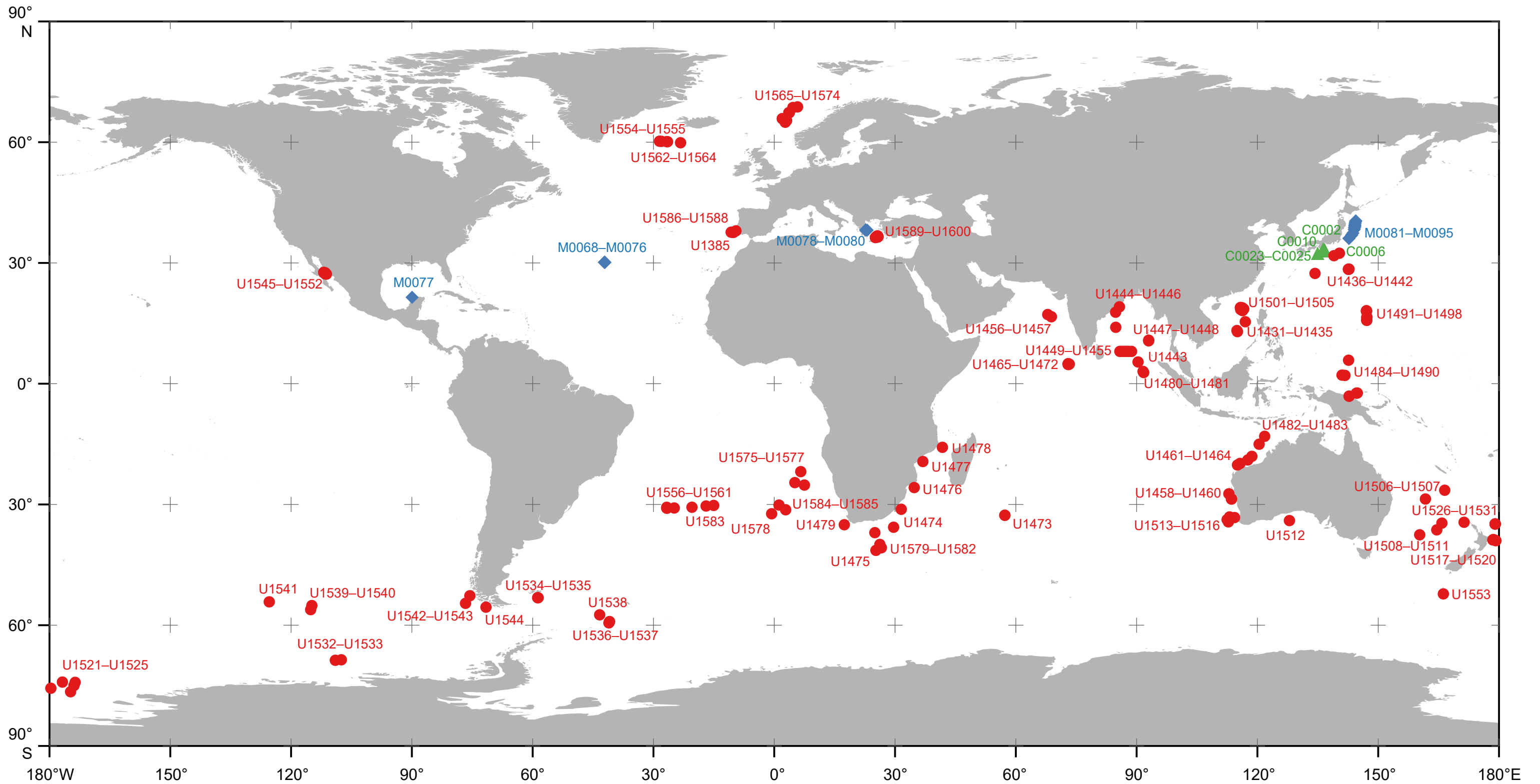
IODP Expeditions 349–372, 374–376, 378–386, 390–393, 396–398, Sites C0002, C0006, C0010, C0023–C0025 (▲), M0068–M0095 (◆), U1385, U1431–U1600 (●)
