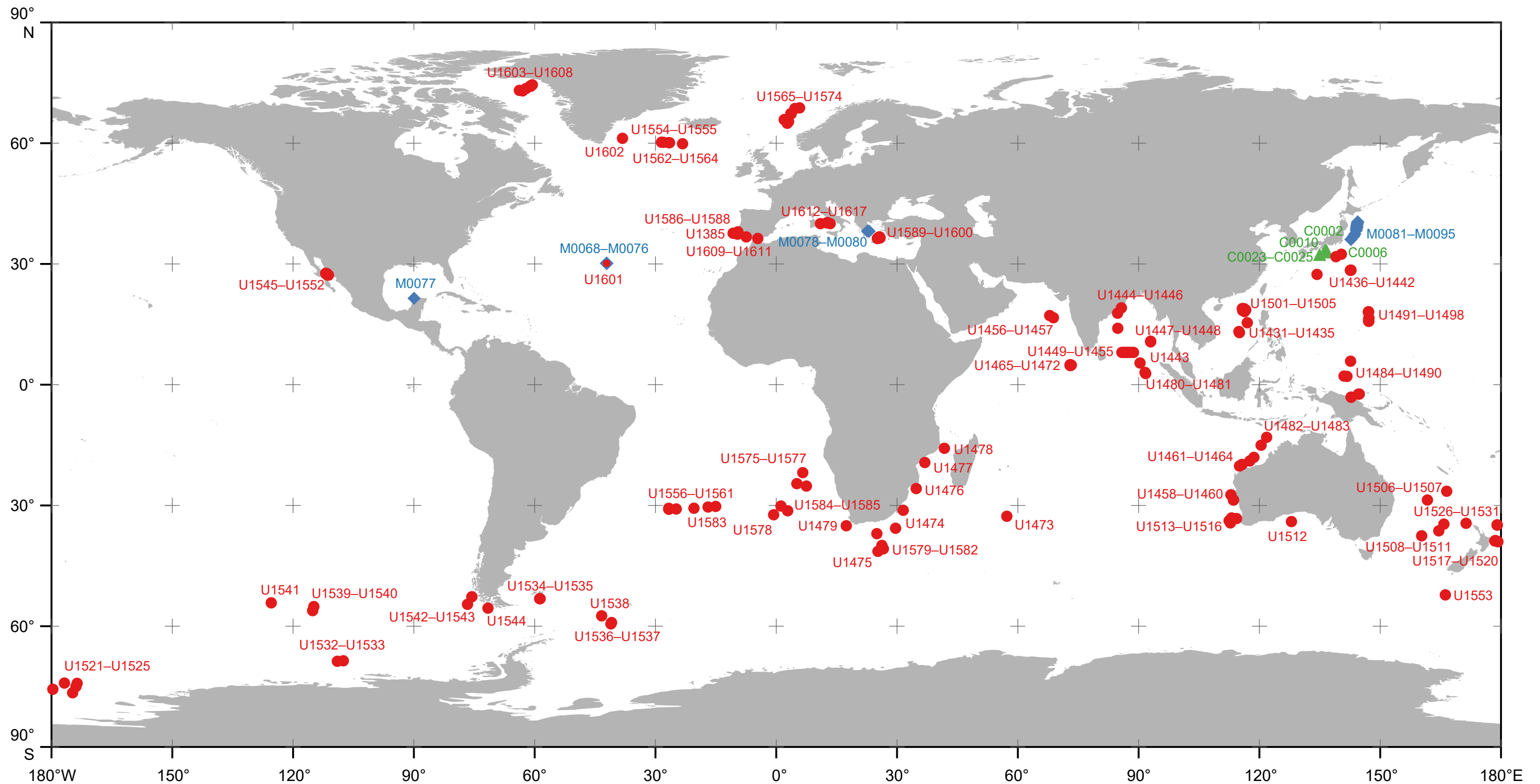
IODP Expeditions 349–372, 374–376, 378–386, 390–393, 395–402, Sites C0002, C0006, C0010, C0023–C0025 (▲), M0068–M0110 (◆), U1431–U1617 (●)
