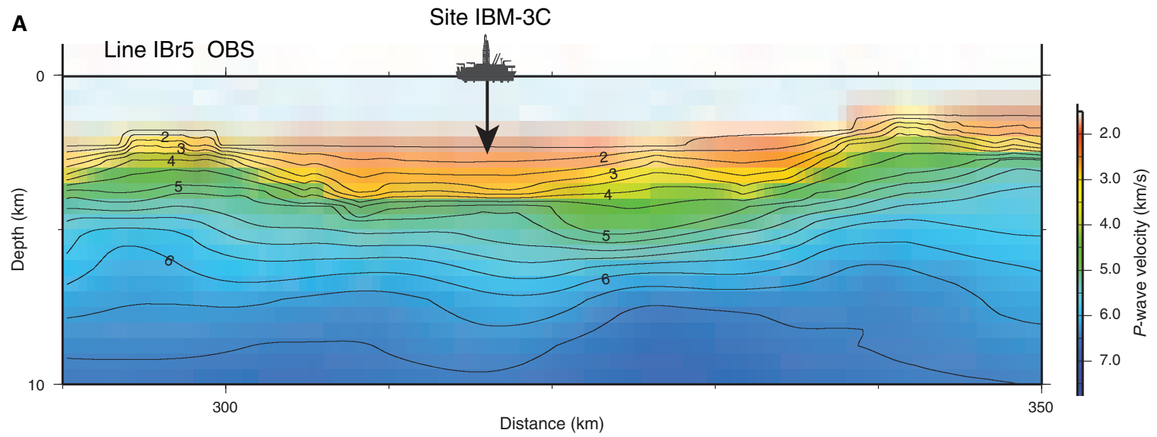
Figure F14. A. Seismic velocity image obtained from wide-angle ocean-bottom seismometer (OBS) data. OBSs are deployed every 5 km along Line IBr5. (Continued on next page.)
