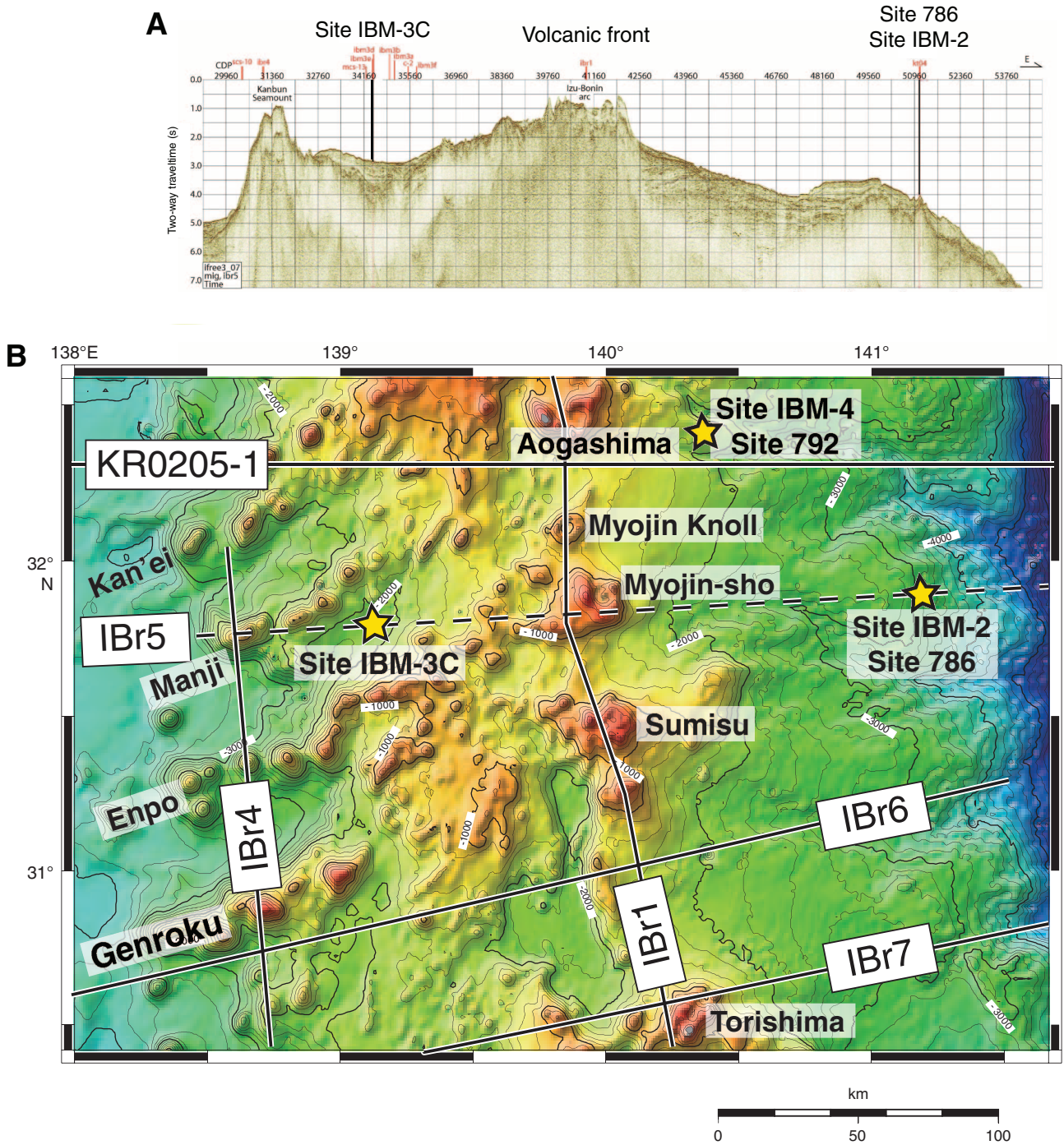
Figure F8. A. Multichannel seismic Profile IBr5 (unpubl. data, JAMSTEC, 2007), uninterpreted time section. Common depth point (CDP) interval = 12.5 m. Vertical exaggeration = ~10. B. Locations of multichannel seismic reflection (MCS) data.
