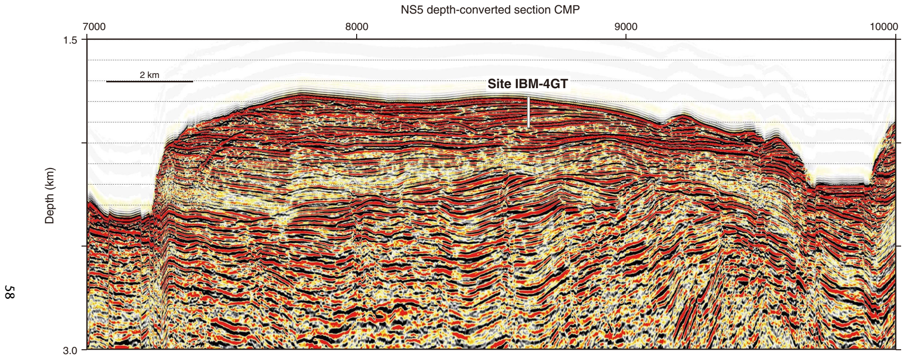
Figure AF4. Seismic reflection profile with location of proposed Site IBM-4GT on Line IBM4-NS5, obtained on Cruise KR08-09. CMP = common midpoint.
