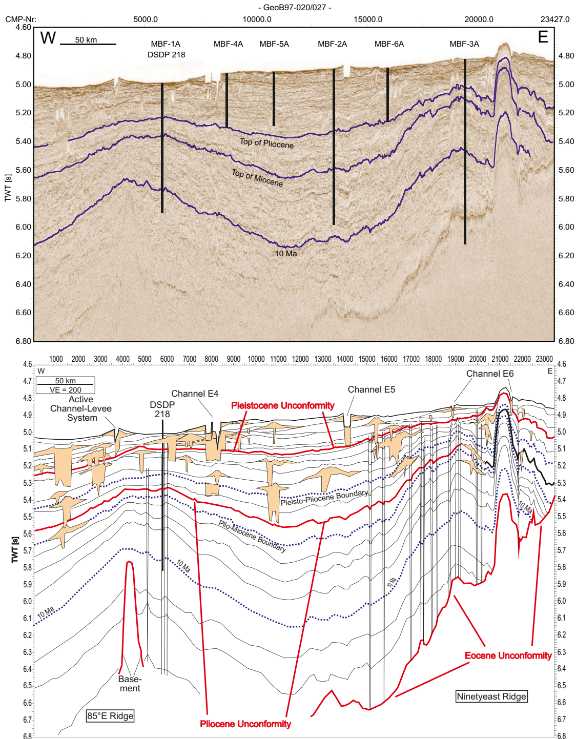
Figure F2. Top: Seismic Profile GeoB097-020/027 showing the positions of Expedition 354 drill sites in relation to regional fan architecture. The tops of the Pliocene and Miocene, as well as the 10 Ma horizon, are traced through the profile based on results from DSDP Site 218 (Moore et al., 1974). The distinct unconformity in the east that is penetrated only by the deepest part of proposed site MBF-3A is inferred to represent the Eocene onset of fan deposition. Bottom: Interpreted line drawing of Profile GeoB97-020/027 showing the later stage channel-levee systems, regional unconformities and faults. Modified from Schwenk and Spieß (2009). TWT = two-way traveltime, VE = vertical exaggeration. Horizontal scale = common midpoint (CMP) numbers, CMP distance = 20 m. Naming of channels follows Curray et al., 2003.
