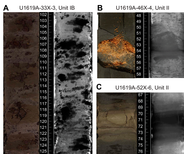
Figure F4. Paired core photographs (left) and X-radiographs (right; black = high-density) showing authigenic minerals, Site U1619. A. Iron sulfide nodules in dark gray (5Y 4/1) silty clay. B. Yellowish orange sand-sized carbonate grains concentrated in lenses within gray (5Y 5/1) silty clay. C. Light brownish gray (2.5Y 6/2) carbonate-rich clayey-silt interval (70–74 cm) that is denser than apparent on the X-radiograph between very dark gray (5Y 3/1) silty clay.
