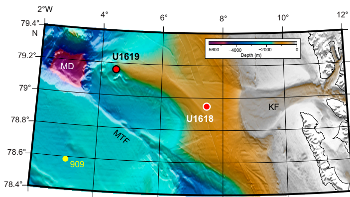
Figure F1. Bathymetric map showing the locations of Sites U1619 and U1618 on the western and eastern terminations of the Vestnesa Ridge sediment drift, respectively. Site U1619 is located ~66 km from Site U1618. The Molloy Transform Fault (MTF) is parallel to and south of the Vestnesa Ridge and connects the actively spreading Knipovich and Molloy Ridge segments. ODP Site 909 is located on an abyssal hill south of the MTF. KF = Kongsfjorden glacial trough. MD = Molloy Deep.
