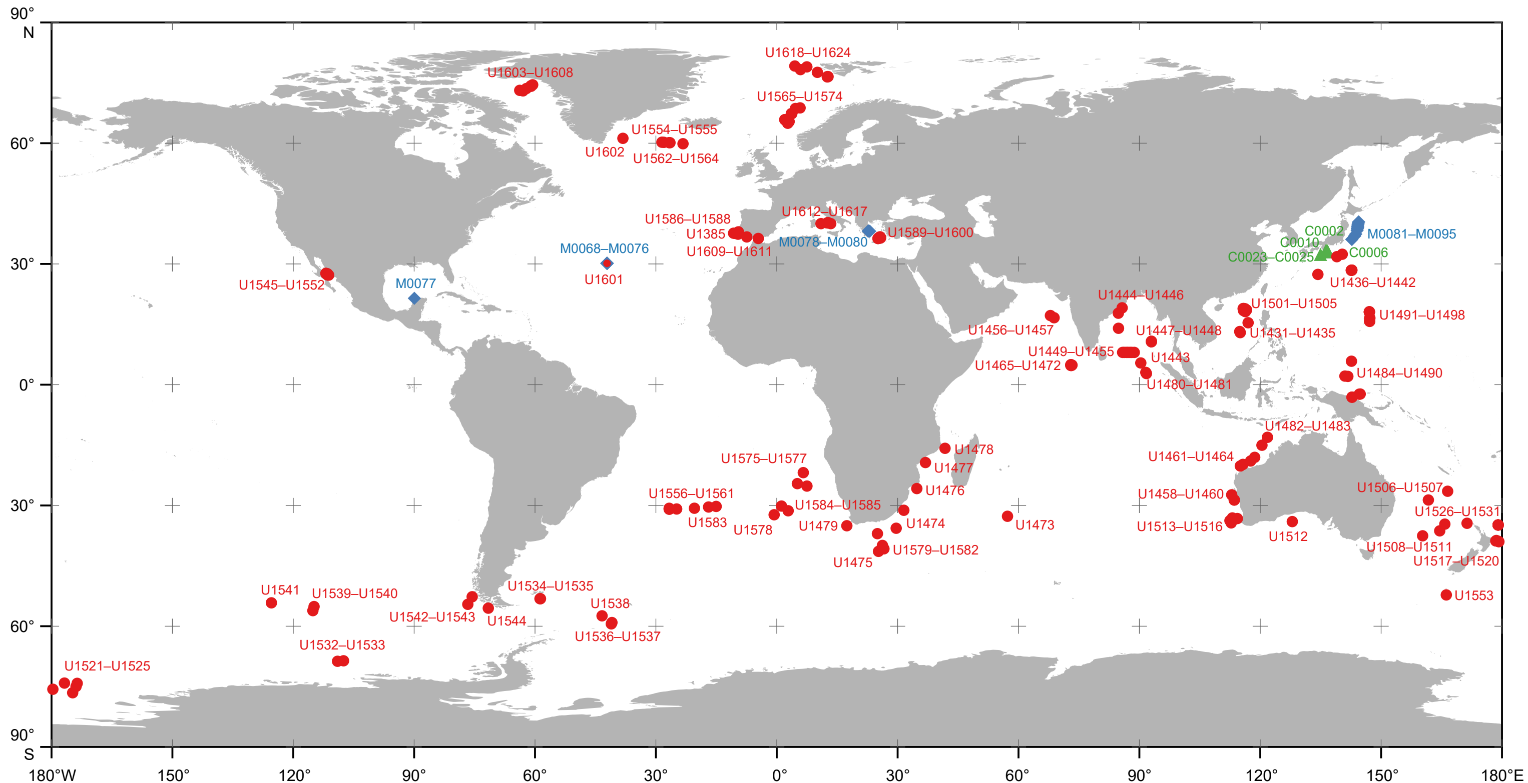
IODP Expeditions 349–372, 374–376, 378–386, 389–393, 395–403, Sites C0002, C0006, C0010, C0023–C0025 (▲), M0068–M0110 (◆), U1431–U1624 (●)
